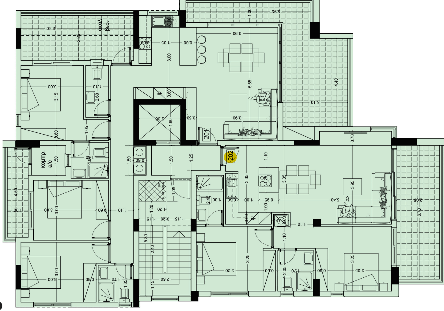
SECOND FLOOR
